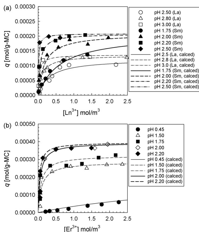
Fig. 1. Extraction isotherms for lanthanum, samarium and erbium with a microcapsule and calculated lines based on Langmuir model: (a) lanthanum and samarium; (b) erbium.
